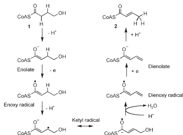
Scheme 1. Proposed mechanism for the dehydration of 4-hydroxybutyryl-CoA ( 1 ) to crotonyl-CoA ( 2 ).
