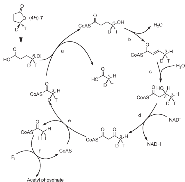
Scheme 3. Conversion of ( R )-4-hydroxy[4- 2 H 1 , 3 H]butyrate into ( S )-[ 2 H 1 , 3 H]acetic acid. Under the conditions of isolation (H + , 100 °C) acetylphosphate was hydrolyzed to acetic acid. The incubation mixture contained hydrolyzed lactone, potassium phosphate pH 7.4, NAD + , acetyl-CoA, CoASH, 4-hydroxybutyrate CoA-transferase (a), 4-hydroxybutyryl-CoA dehydratase (b), crotonase (c), ( S )-3-hydroxybutyryl-CoA dehydrogenase (d), thiolase (e), and phosphotransacetylase (f).
