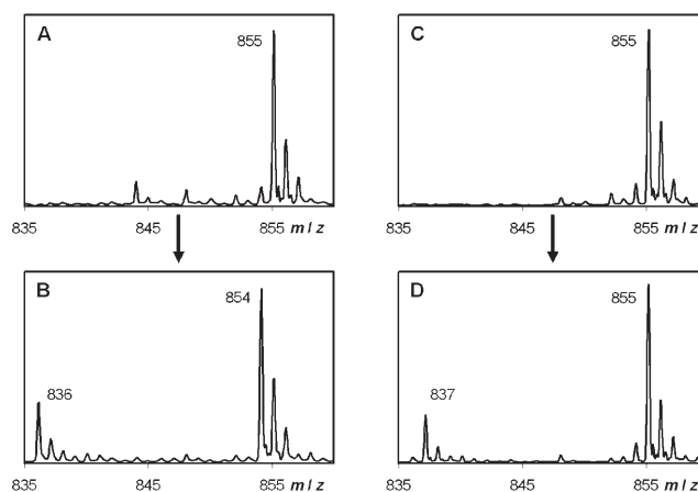
Figure 1. MALDI-TOF mass spectra. A) (2 R )- 1 (855 Da); B) upon incubation of (2 R )- 1 with dehydratase, loss of deuterium in the product crotonyl-CoA ( 2 , 836 Da) and exchange by hydrogen in 4-hydroxybutyryl-CoA ( 1 , 854 Da) are observed; C) (2 S )- 1 (855 Da); D) upon equilibration with dehydratase, (2 S )- 1 retains the deuterium, and [2- ^2\text{H} ]crotonyl-CoA (837 Da) is formed.
